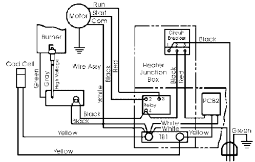
4 Wire PC Board Wiring Diagram
